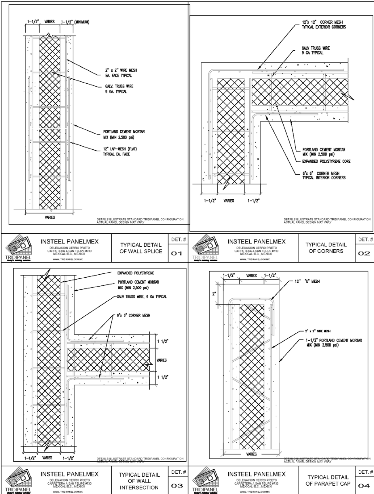
FIGURE 13—TYPICAL INSTALLATION DETAILS
